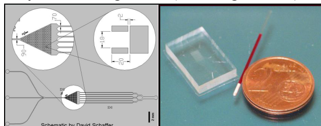
Figure 1: Left Panel – Schematic of the multitrap nanophysiometer (MTNP). 440 traps (inset) are arrayed in a 2 x 2 mm chamber with three inputs and one output. Right Panel – The MTNP device with a €0.02 (U.S. penny-sized) coin and a glass microtube containing 10 microliters of whole blood.
