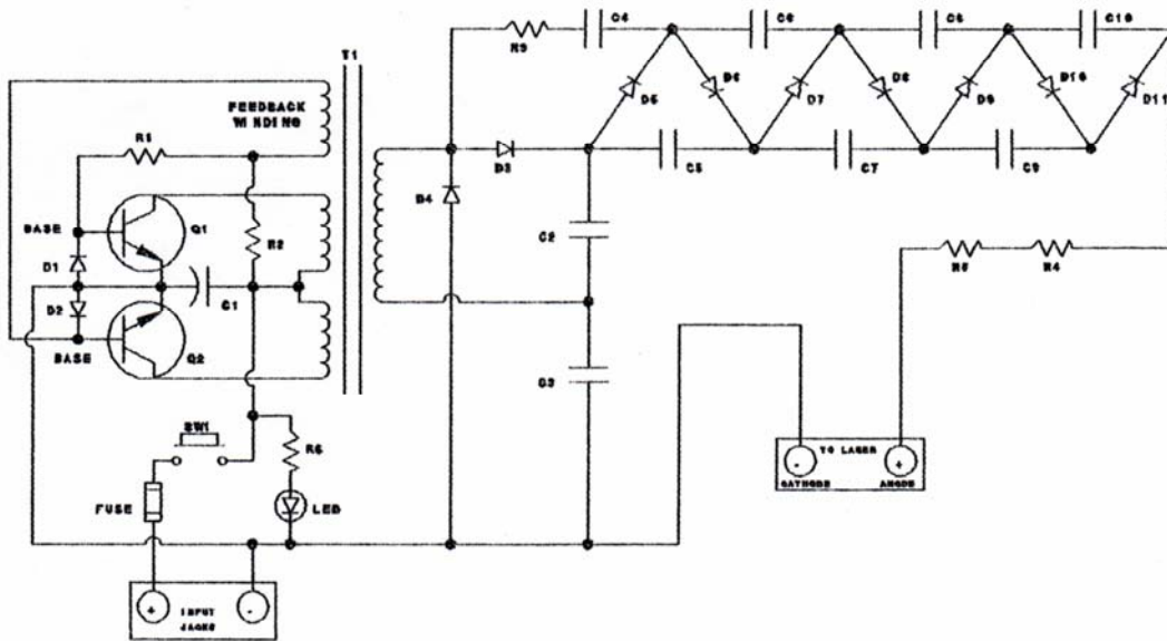
Figure 5: Laser power supply circuitry
