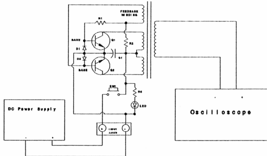
Figure 6: Connections to test transistor inverter
